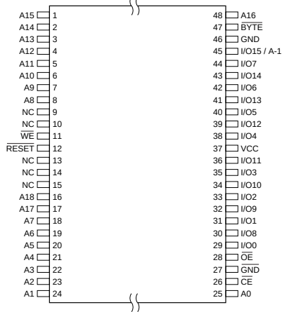
AT49F8192A(T) TSOP Top View Type 1
